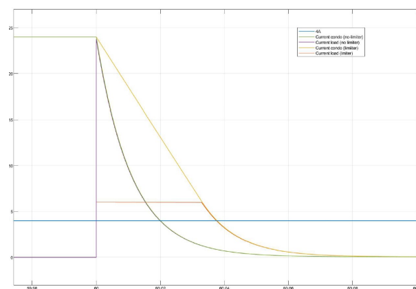
FIGURE 5.8 – Simulation matlab
